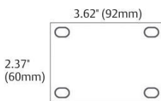
Top view of caster plates
